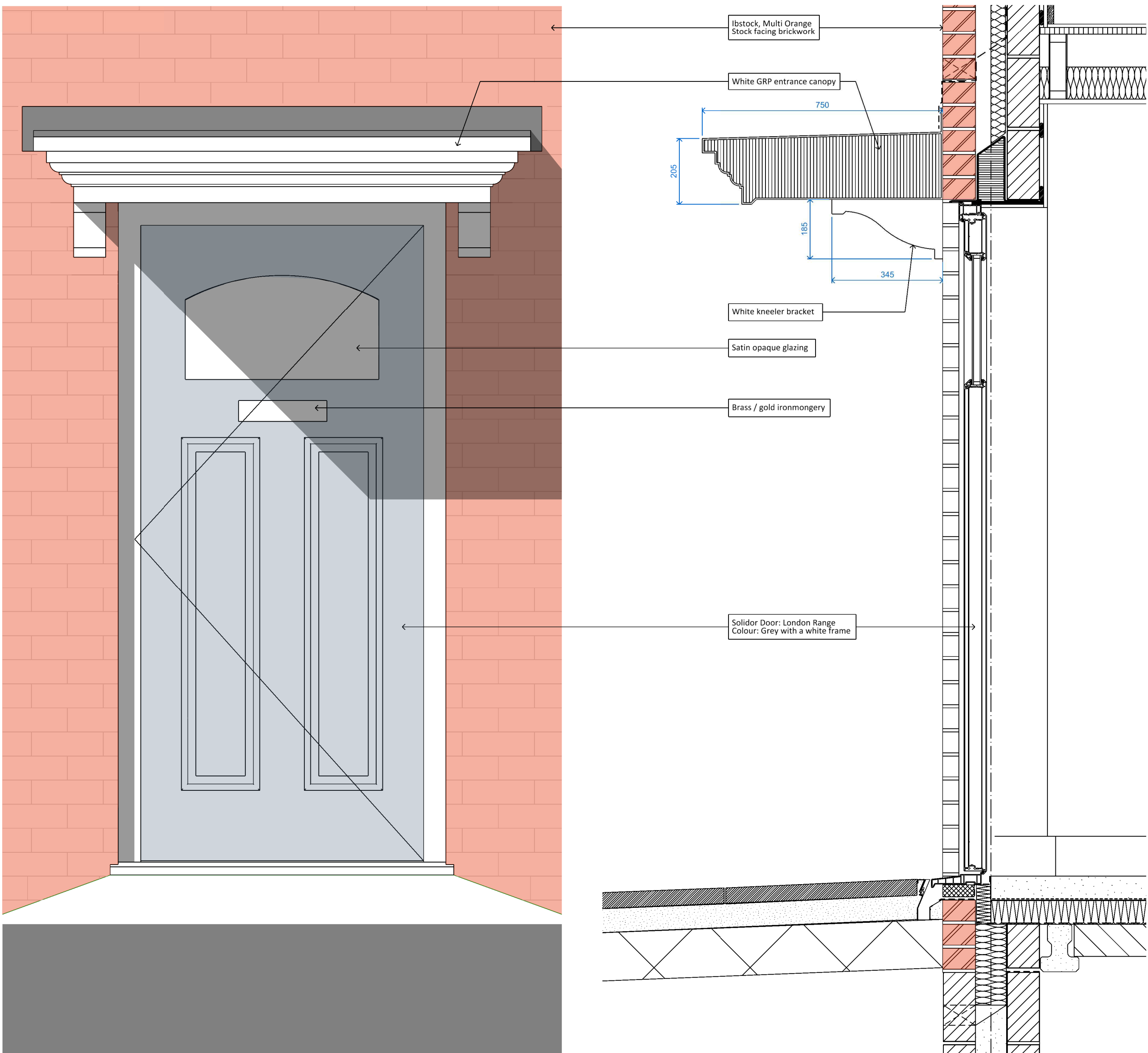
E06 Front Door & Canopy Elevation (Scale 1:10 @ A1)
