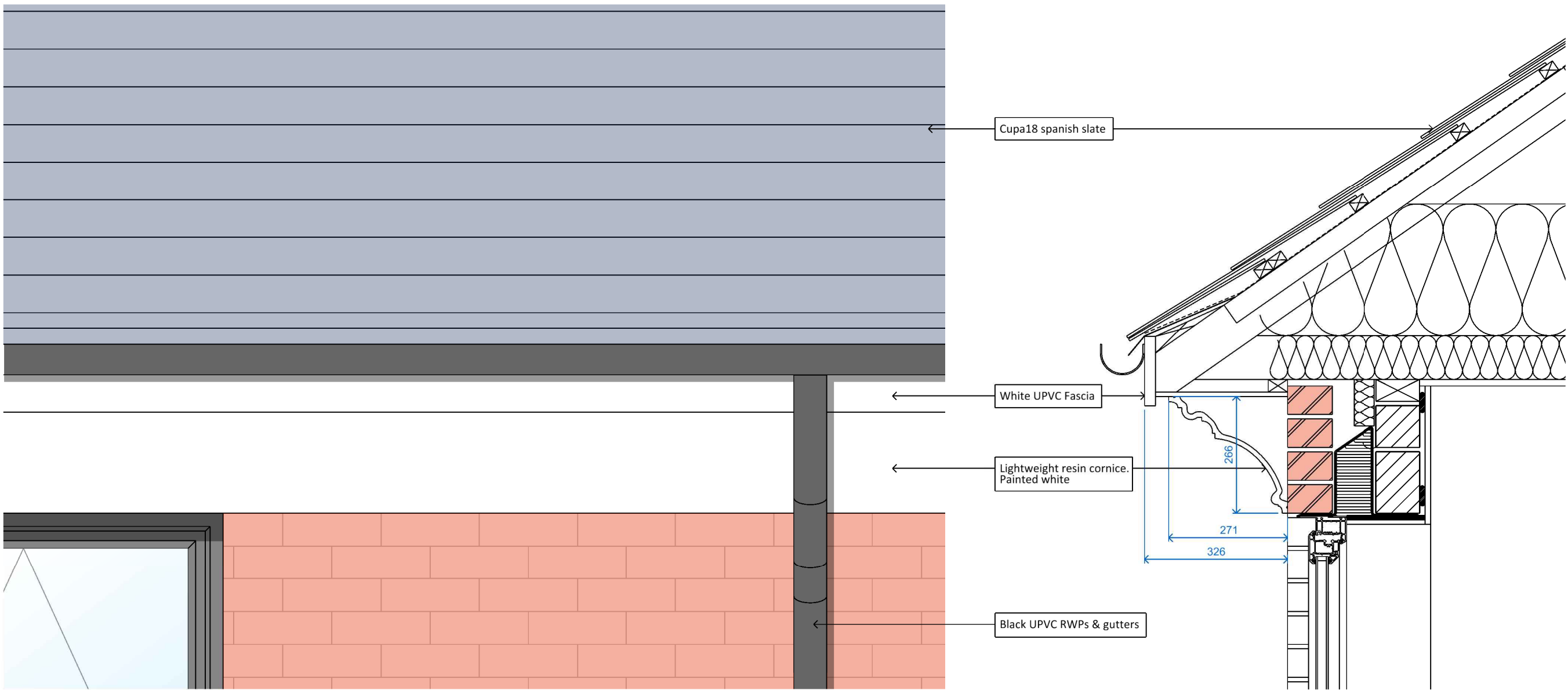
E07 Eaves, RWPs & Gutter Elevation (Scale 1:10 @ A1)
